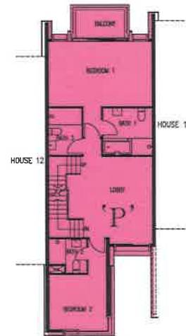
1/F Plan
